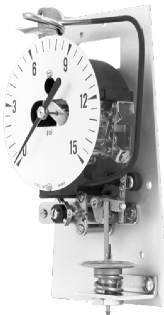
Model 40 Pneumatic Transmitter
