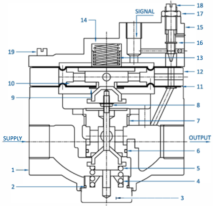
Figure 2. Sectional View PHVB-03/04/05/06
