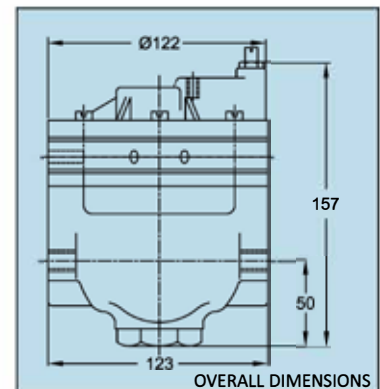
OVERALL DIMENSIONS
