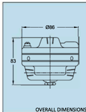
OVERALL DIMENSIONS
