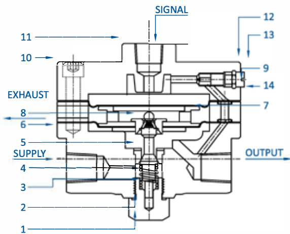
Figure 1. Sectional View Model PHVB-01/02
